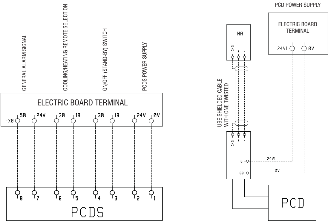
DIAGRAM SHOWING ELECTRICAL CONNECTIONS BETWEEN MPE AND PCDS / PCD REMOTE CONTROL PANEL
