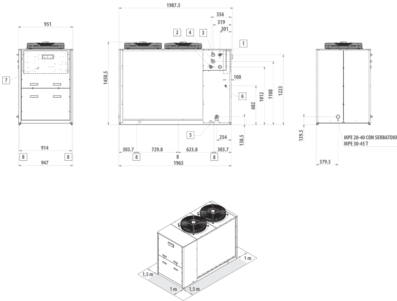
MPE 28-45 WITH BUFFER TANK MPE 30-45 T
