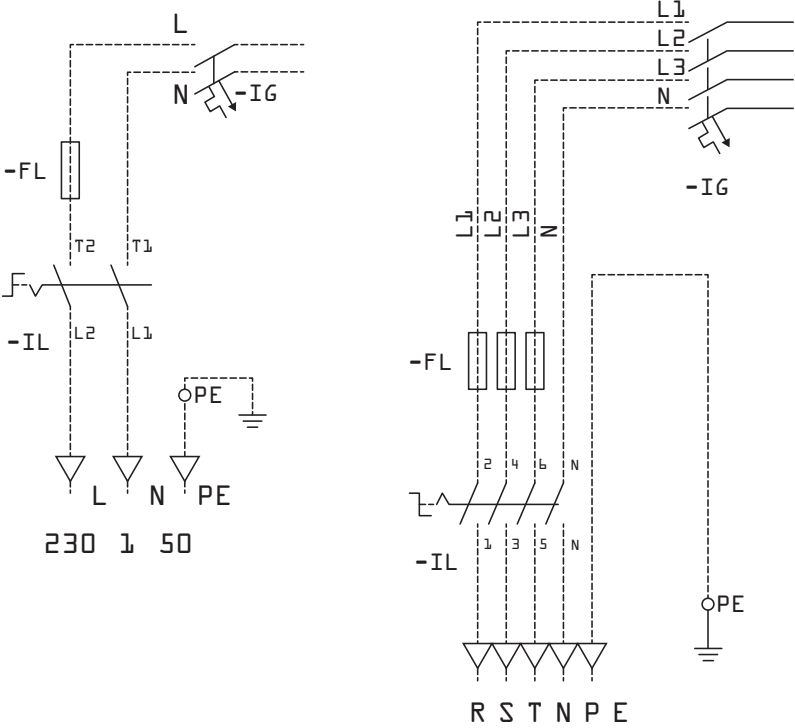
DIAGRAM SHOWING ELECTRICAL CONNECTIONS BETWEEN MPE AND PCDS / PCD REMOTE CONTROL PANEL
